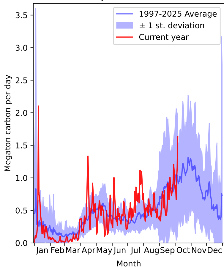
Daily fire emissions
