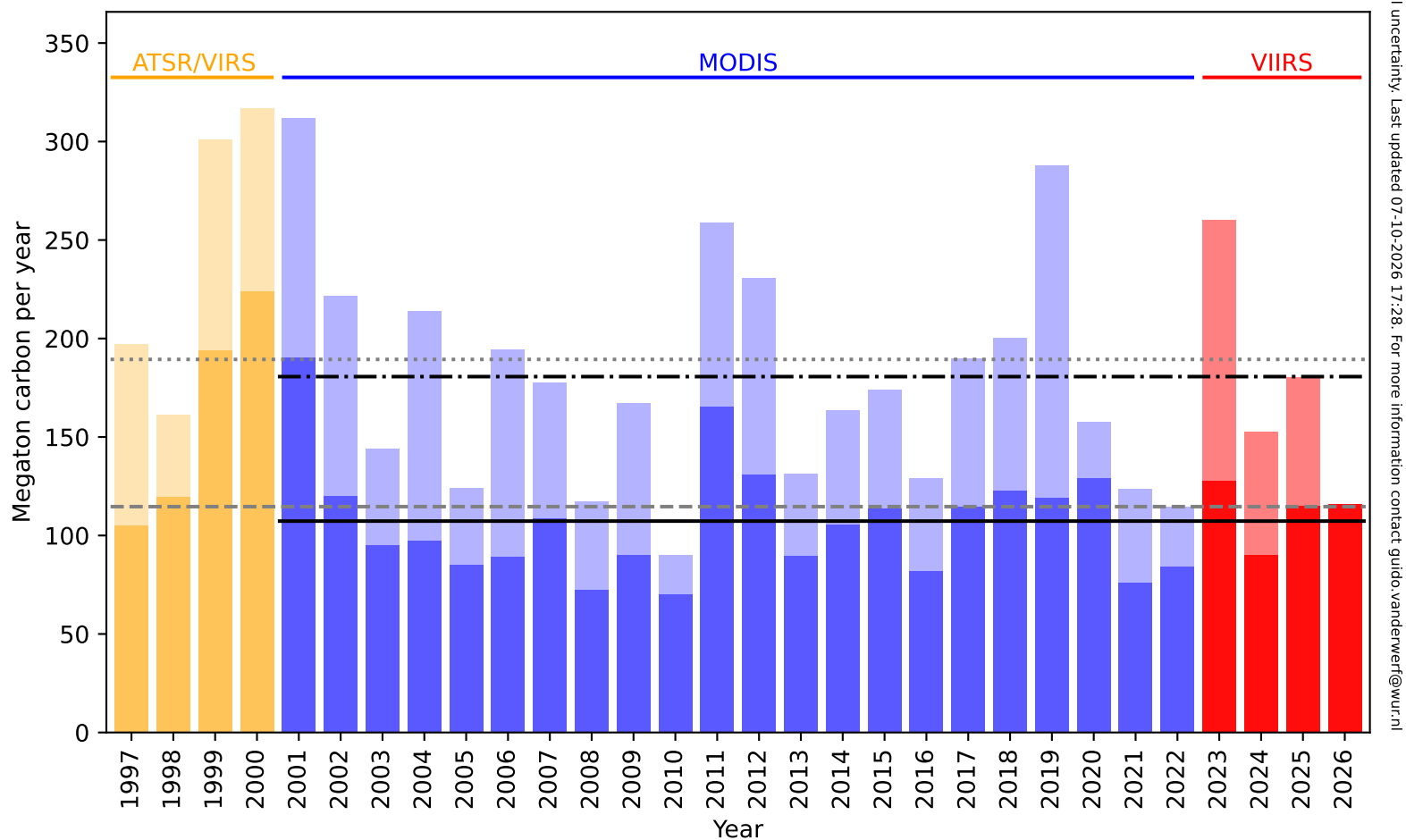
Annual fire emissions
