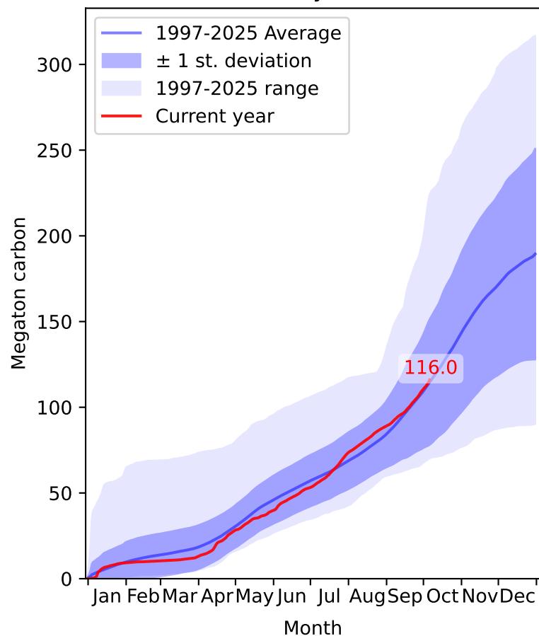
Cumulative daily fire emissions
