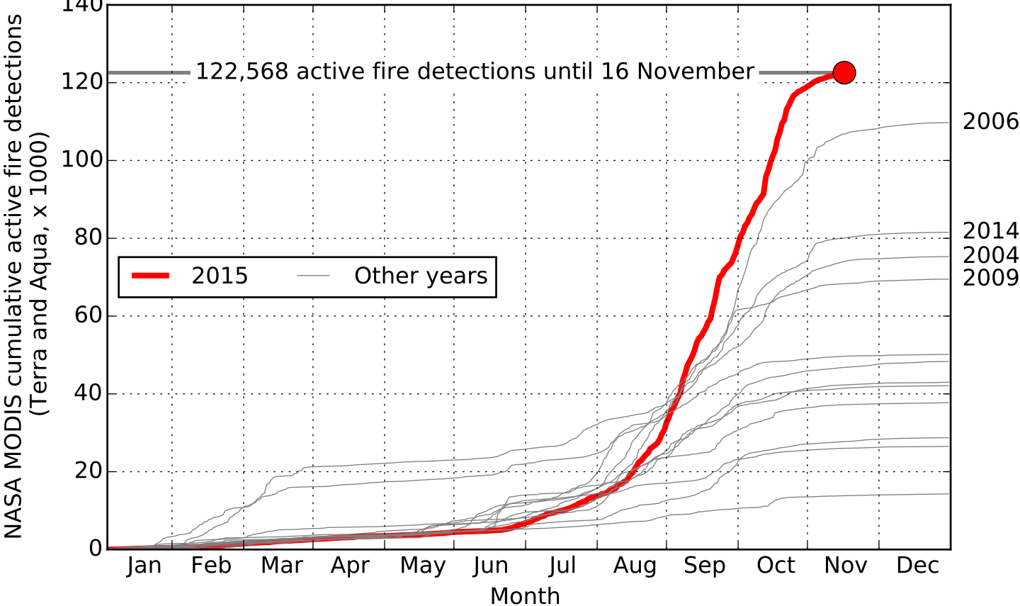
Satellite-based active fire detections over Indonesia (2003-2015)
